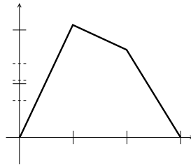
FIGURE 2. Global roof function
