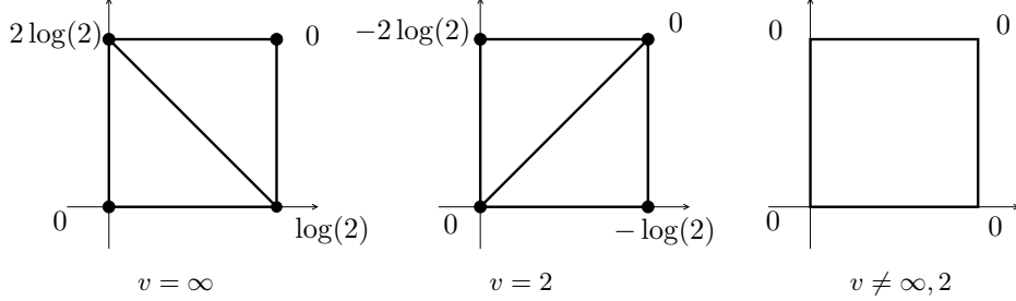
FIGURE 3. Local roof functions
