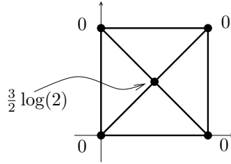
FIGURE 4. Global roof function
