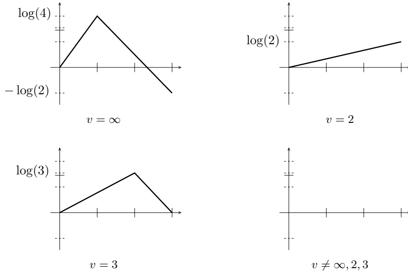
FIGURE 1. Local roof functions
