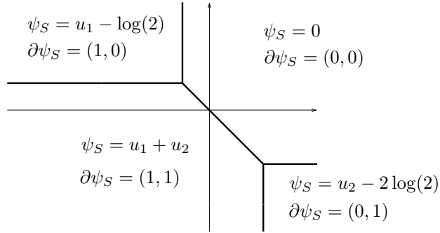
FIGURE 5. Function \psi_S and its gradient
